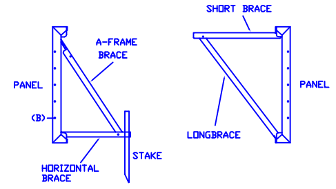
A-FRAME DETAIL DECK SUPPORT DETAIL
